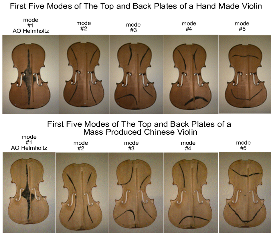
Figure 4.02 First Five Signature Modes are the Same on All Violins (Reprinted with permission from Emmanuel Bossy, and Renaud Carpentier, (Physics Department, University of Southern Wales, Australia), cropped, http://www.phys.unsw.edu.au/jw/patterns1.html and http://www.phys.unsw.edu.au/jw/patterns2.html .) Copyright 2006, University of South Wales.)
